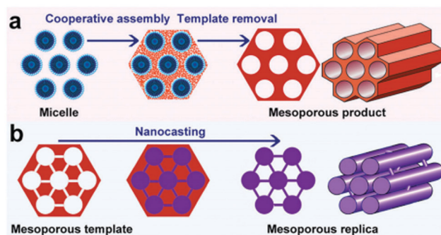
Fig. 16 (a) soft-templating and (b) hard-templating synthesis routes for the design of ordered mesoporous materials. Reproduced with permission from ref. 166. Copyright (2011) Royal Society of Chemistry.
