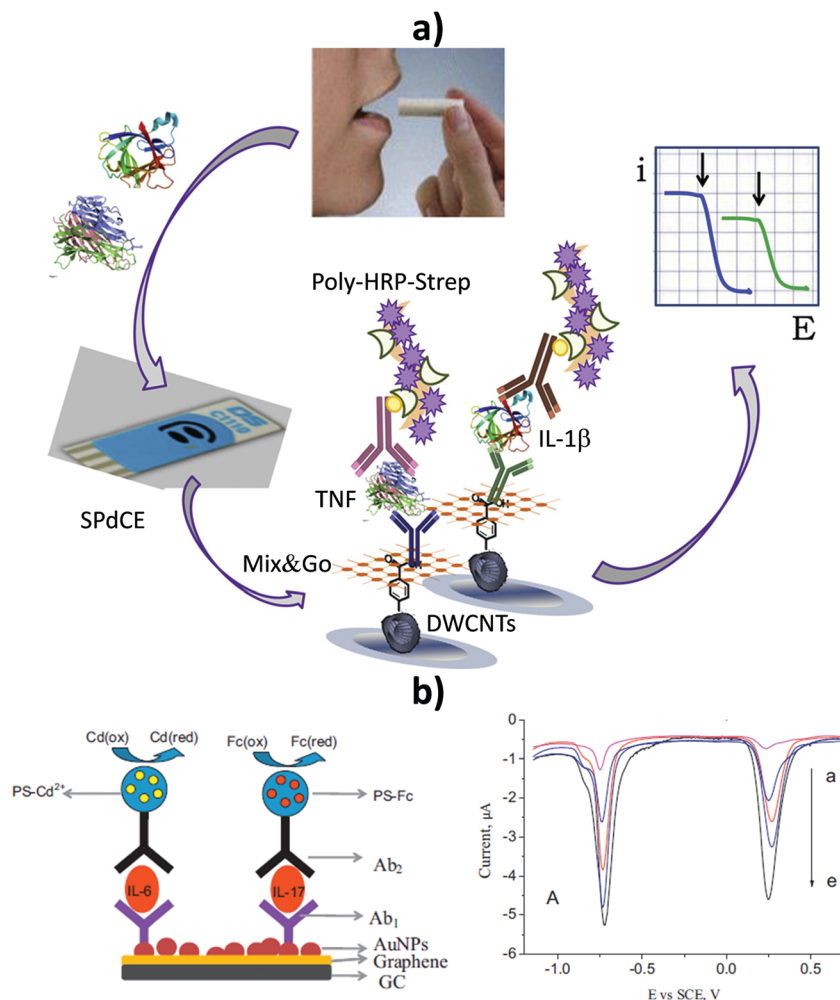
Fig. 16 Multiplexed electrochemical sandwich immunoplatforms using (a) multielectrode arrays or (b) barcode configurations. Simultaneous amperometric determination of TNF and IL-1 \beta at a SPdCE modified with 4-carboxyphenyl-functionalized double-walled carbon nanotubes (HOOC-Phe-DWCNTs) and polymeric coating Mix&Go to immobilize the capture antibodies in an oriented manner (a). Schematic illustration of the bioplatfrom developed for the simultaneous SWV determination of IL-6 and IL-7 using polystyrene spheres (PS) containing Cd 2+ or ferrocene (Fc) as tags (b, left). SWV traces recorded for simultaneous determination of increasing concentrations of IL-6 and IL-17 standards (b, right; from (a) to (e): 5, 50, 100, 500, 1000 \mu\text{g mL}^{-1} ). Reproduced and adapted from (a) ref. 19 and (b) ref. 184 with permission.
