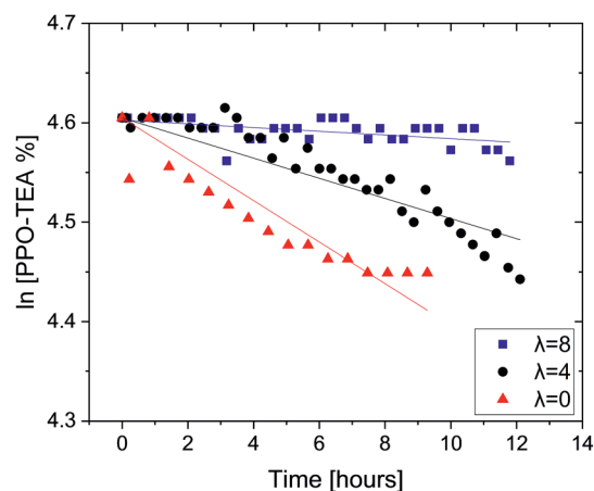
Fig. 2 Remaining PPO-TEA fractions as a function of time with hydration number \lambda = 0, 4 and 8 , in 0.06 \text{ M OH}^- DMSO- d_6 solutions. All tests were done at room temperature.
