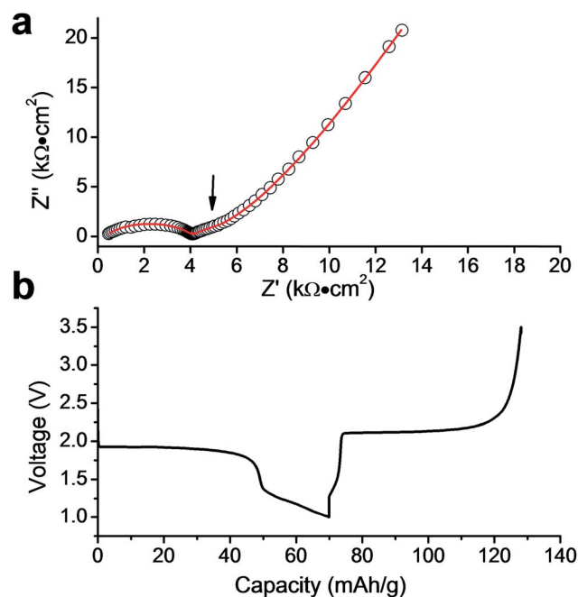
Fig. 9 (a) The impedance spectrum collected from the Li/LZF/LTP cell (LZF pellet thickness \sim 0.9 mm) at 50 °C; the arrow indicates an intermediate-frequency semicircle assigned to the LTP/LZF interfacial resistance. (b) Discharge/charge profile of the Li/LZF/LTP cell at 50 °C and 6 \mu\text{A cm}^{-2} .
