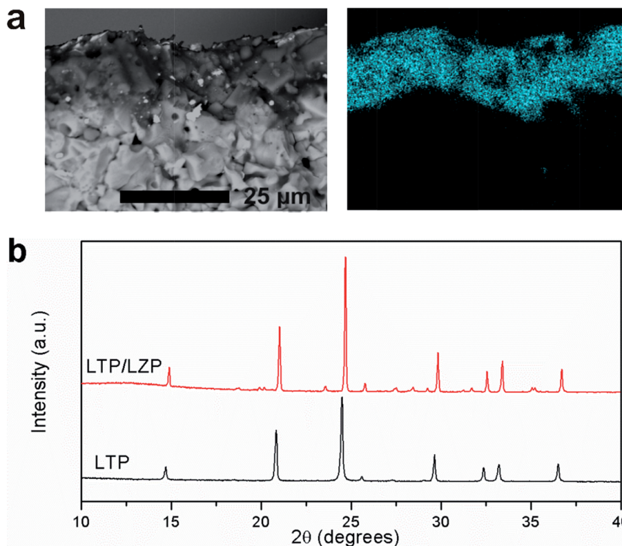
Fig. 8 (a) SEM image of a longitudinal section of the LZF-1100 pellet after depositing LTP, collected using AsB detector, and an EDX elemental map of the sample showing the distribution of Ti (blue). (b) XRD pattern of as-prepared LTP powder, and XRD pattern collected from the LZF pellet surface after depositing LTP.
