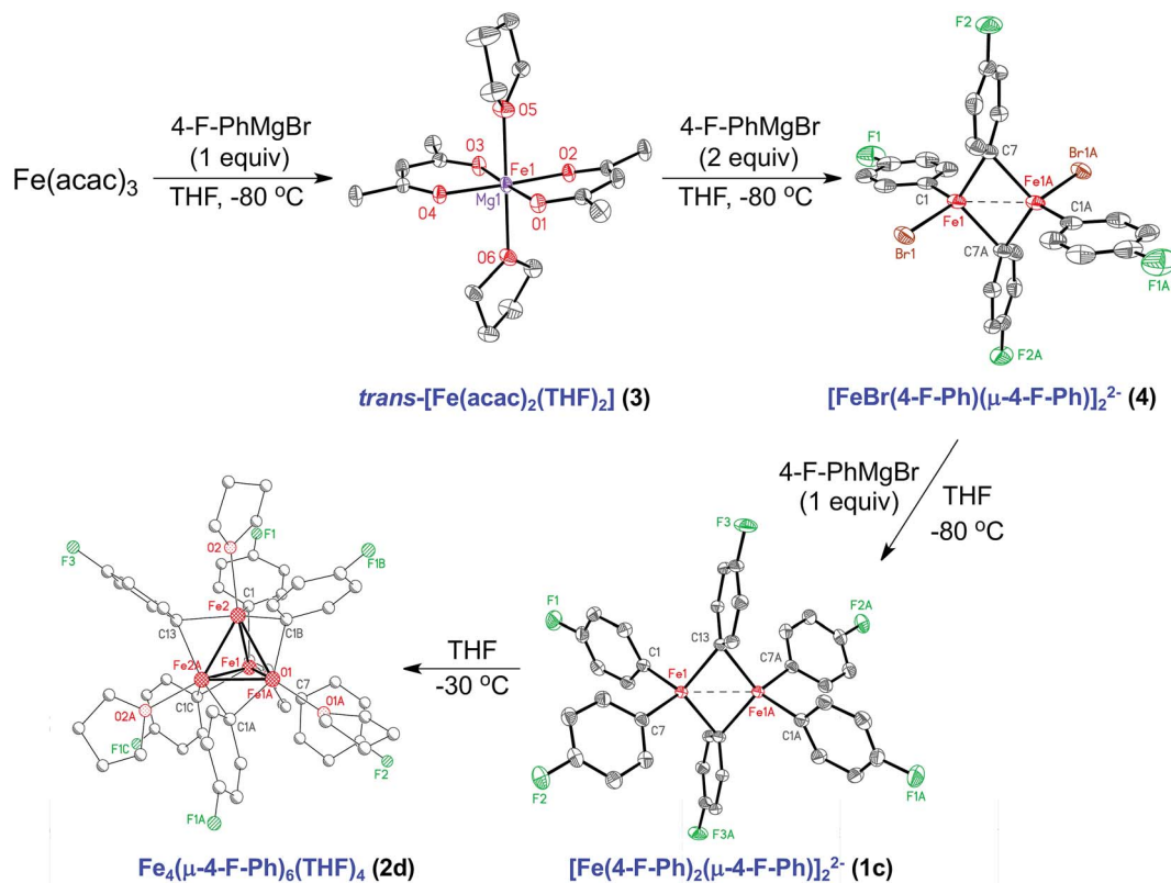
Fig. 4 Iron species in the synthetic pathway for the formation of tetranuclear iron-aryl species utilizing \text{Fe}(\text{acac})_3 and 4\text{-F-PhMgBr} . Hydrogen atoms omitted for clarity and thermal ellipsoids are shown at 50% probability for 1c , 3 and 4 .
