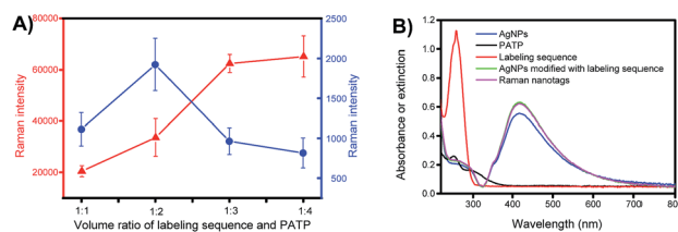
Fig. 4 (A) Comparison of signals for Raman nanotags prepared with labelling sequence solution ( 10\ \mu\text{M} ) and PATP solution ( 100\ \mu\text{M} ) at different volume ratios on a gold-coated substrate (red) and on a target miRNA-bond extraction sequence-modified gold-coated substrate (blue). Error bars represent standard deviations. (B) UV-visible absorption spectra for PATP and the labelling sequence and UV-visible extinction spectra for AgNPs, AgNPs modified with labelling sequence (without a Raman reporter) and Raman nanotags.
