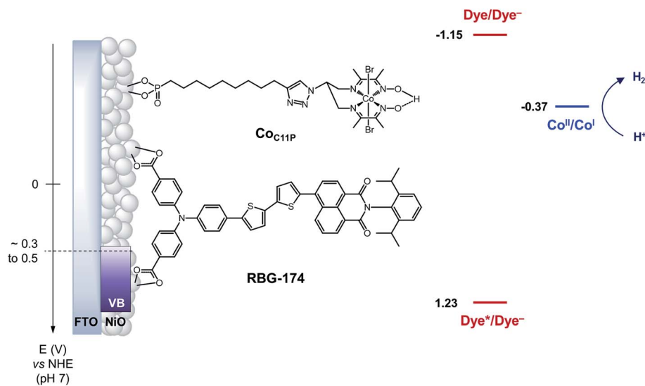
Fig. 1 Schematic energy diagram of the NiO/IRBG-174/CoC 11 P photocathode. See text for the estimation of energy levels at pH = 7. Potentials for the redox couples of RBG-174 have been determined as described in ref. 48 from data found in ref. 40.
