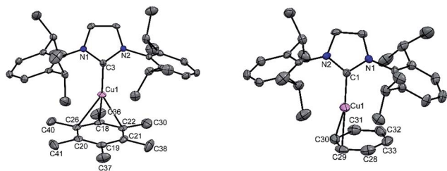
Fig. 3 Molecular structure of 5 and 6 (ellipsoids are shown at the probability level of 50%). Counter anion SbF 6 - and hydrogen atoms are omitted for clarity. Selected bond lengths (Å) 5 : N1–C3 1.353(4), N2–C3 1.356(4), Cu1–C3 1.890(3), Cu1–C18 2.114(4), Cu1–C22 2.289(4), Cu1–C26 2.319(4), Cu1–C21 2.678(4), Cu1–C20 2.715(4), and Cu1–C19 2.894(4). 6 : C1–N1 1.356(7), C1–N2 1.349(6), C1–Cu1 1.886(5), Cu1–C29 2.129(6), Cu1–C30 2.217(5), Cu1–C28 2.456(6), Cu1–C31 2.621(5), Cu1–C33 2.813(6), and Cu1–C32 2.892(6).
