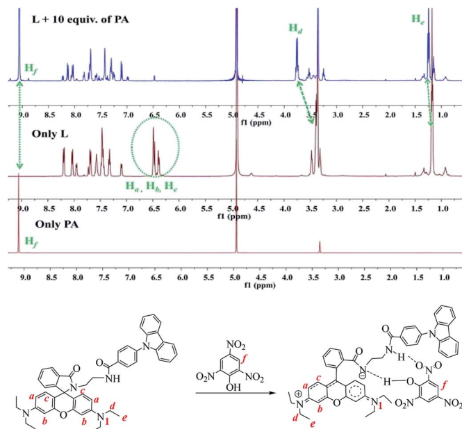
Fig. 9 ^1\text{H} NMR spectra of L, PA and the mixture of L + PA in \text{CD}_3\text{OD} .
