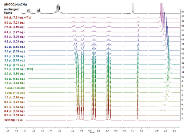
Fig. 4 Stacked 1 H NMR spectra (thf-d 8 ) of a titration experiment of [(\{NCOC_6H_4\}_2CH)K(thf)]_n ( 2 ) with water and a free uncharged ( \{NCOC_6H_4\}_2CH_2 ) ligand (black).
