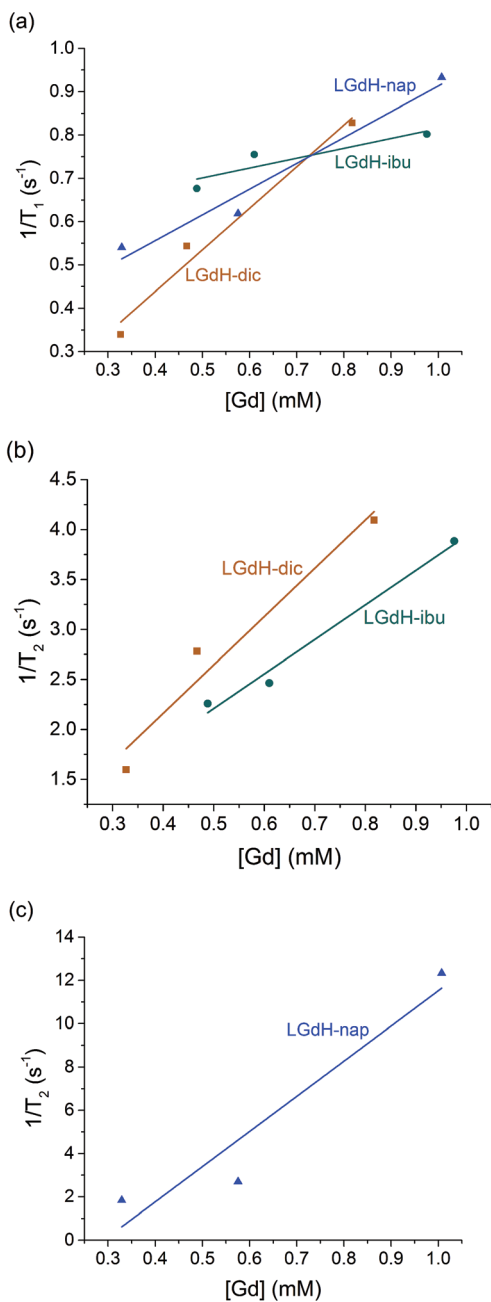
Fig. 9 Relaxivity data on the LGdH-drug composites prepared by ion exchange, showing (a) r_1 , (b) and (c) r_2 plots.
