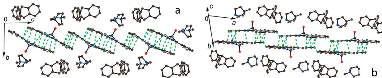
Fig. 11 View along the phthalocyanine layers composed of the \{Ti^{IV}(O)(Pc^{\cdot 3-})\}_2 dimers in 12 : view along the a (a) and approximately along the c (b) axes. Short van der Waal contacts between phthalocyanines are shown by green dashed lines.
