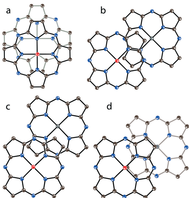
Fig. 12 View of the \pi -stacking \{Ti^{IV}(O)(Pc^{\cdot 3-})\}_2 dimers along the M=O bonds: (a) optimal overlapping observed in 1 , 8 and 13 ; (b) partial overlapping observed in 2 ; (c) weak overlapping observed in 4 and 9 ; (d) intermediate overlapping in 12 . Only 24-atom Pc planes are shown.
