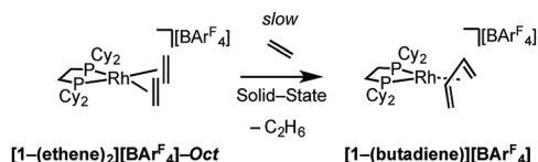
Scheme 5 Dehydrocoupling of [1-(\text{ethene})_2][\text{BAr}^{\text{F}}_4] .
