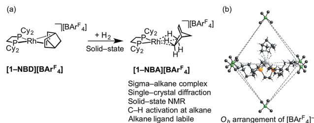
Scheme 2 (a) Synthesis of sigma-alkane complex [1-NBA][BAR F 4 ] by solid/gas reactivity; (b) O n arrangement of [BAR F 4 ] anions in the solid-state that encapsulate cation (Ar F groups removed).
