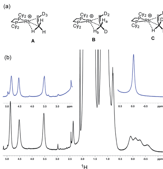
Scheme 9 (a) Isotopomers [1-(d_3\text{-propene})][\text{BAR}^F_4] highlighting the methyl substitution patterns. (b) ^1\text{H} NMR spectra (193 K, \text{CD}_2\text{Cl}_2 ) of a sample prepared by the solid/gas route after 16 hours. Top, [1-(\text{propene})][\text{BAR}^F_4] ; bottom, [1-(d_3\text{-propene})][\text{BAR}^F_4] .
