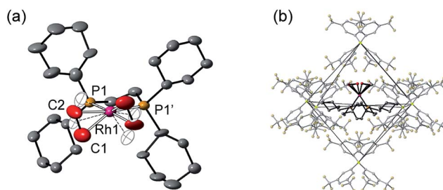
Fig. 1 Solid-state structure of [1-(ethene) 2 ][BAR F 4 ]-Oct . (a) Cation showing the numbering scheme, displacement ellipsoids shown at the 50% probability level, 50% disorder component shown as open ellipsoids. (b) Local environment around the cation showing the arrangement of [BAR F 4 ] − anions. H-Atoms are omitted.
