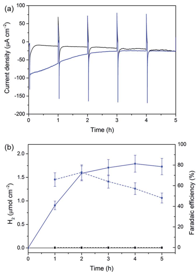
Fig. 5 CPP traces for \text{Si|mesoTiO}_2 (black) and \text{Si|mesoTiO}_2|\text{H}_2\text{ase} (blue) at 0.0 V vs. RHE during continuous illumination with UV-filtered simulated solar light (AM1.5G, 100 \text{ mW cm}^{-2} , \lambda > 400 \text{ nm} ). (a) Chronoamperograms with an hourly dark chop lasting for two min each and (b) \text{H}_2 evolution (solid traces) and cumulative faradaic efficiency (dashed traces). Conditions: aqueous 2-( N -morpholino)ethanesulphonic acid solution (50 mM, pH 6), inert atmosphere, room temperature.
