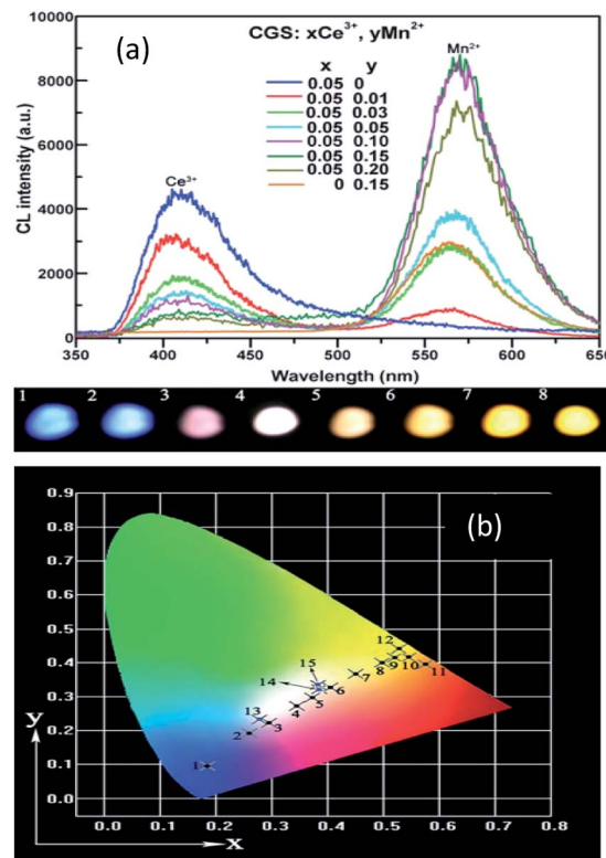
Fig. 15 (a) Emission spectra and luminescence properties of CGS: x\text{Ce}^{3+}, y\text{Mn}^{2+} samples. (b) The CIE chromaticity diagram for \text{Ca}_2\text{Gd}_8(\text{SiO}_4)_6\text{O}_2:0.05\text{Ce}^{3+}, y\text{Mn}^{2+} samples under 287 nm UV excitation. 86
