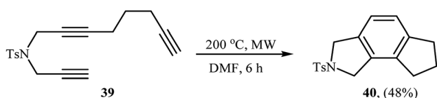
Scheme 14 Formation of 6,7,8-trihydrocyclopenta[5H]isoindoline 40 through non-metal-catalyzed intramolecular alkyne cyclo-trimerization reaction promoted by focussed microwave heating.
