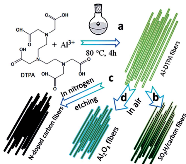
Fig. 29 Schematic illustration of the formation process of the nanoporous N-doped carbon microfibres and solid acids microfibers. [Reproduced from ref. 305 with permission from The Royal Society of Chemistry.]
