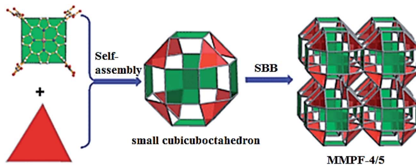
Scheme 8 The scheme of synthesis of MMPF-4 ( M = \text{Zn} ) and MMPF-5 ( M = \text{Cd} ) based on small cubicuboctahedral SBBs. [Reproduced from ref. 59 with permission from The Royal Society of Chemistry.]
