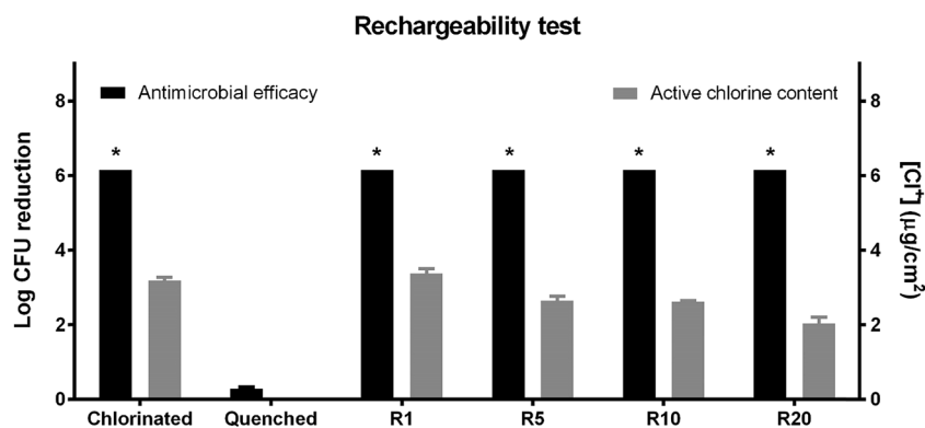
Fig. 5 Antimicrobial efficacies and oxidative chlorine contents of rechargeable N -halamine modified TPU films. Inoculum: E. coli O157:H7 (6.15 log CFU/6.45 \text{cm}^2 ). * indicates a total kill of all inoculated bacteria.
