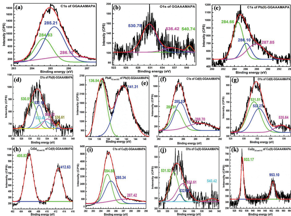
Fig. 5 XPS analyses of C 1s (a, c, f and i), O 1s (b, d, g and j) for GGAAAMAPA and \text{Pb(II)} , \text{Cd(II)} and \text{Cu(II)} adsorbed GGAAAMAPA; \text{Pb } 4f_{7/2} \text{ and } 5/2 (e), \text{Cd } 3d_{5/2} \text{ and } 3/2 (h) and \text{Cu } 2p_{3/2} \text{ and } 1/2 (k) of \text{Pb(II)} , \text{Cd(II)} and \text{Cu(II)} adsorbed GGAAAMAPA, respectively.
