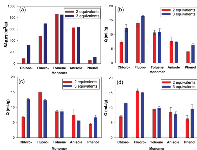
Fig. 4 (a) Apparent SA_{BET} and swellability ( Q ) in; (b) triethylamine, (c) ethyl acetate, and (d) DMF for the HCPs prepared using 2 equivalents and 3 equivalents of FDA as crosslinker.
