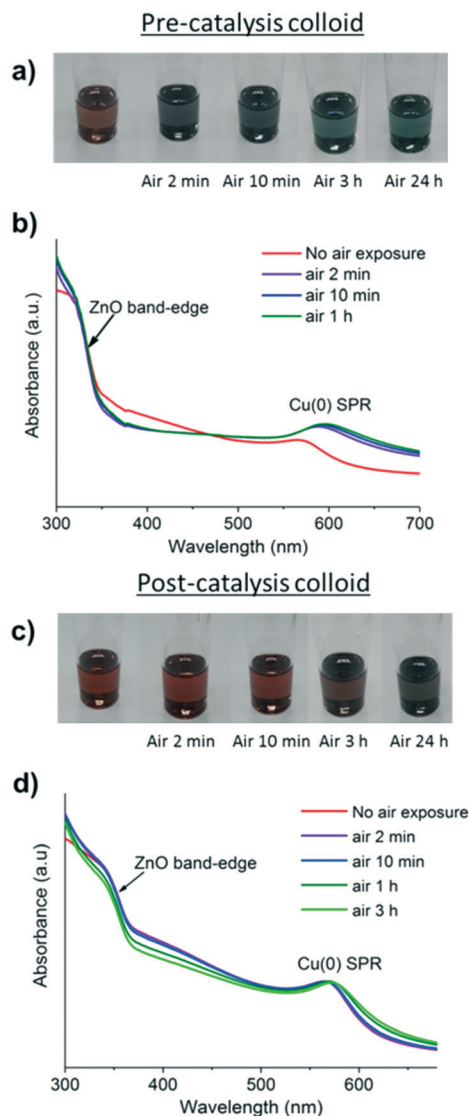
Fig. 6 a & b) Photographs and UV-vis spectra of the pre-catalysis CuMesZnO@DOPA solution before and after air exposure. c & d) Photographs and UV-vis spectra of the CuMesZnO@DOPA post-catalysis solution before and after air exposure.
