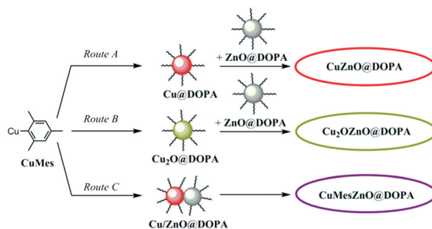
Fig. 1 Synthetic routes to Cu/ZnO pre-catalyst colloids coordinated by the [\text{DOPA}]^- ligand.
