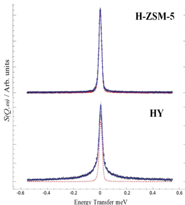
Fig. 13 QENS spectra at 298 K of methanol loaded in zeolites H-ZSM-5 and HY at Q = 0.9 \text{ \AA}^{-1} , (--) represents the resolution data taken at 5 K. Reproduced from ref. 65 with permission of the Royal Society of Chemistry.
