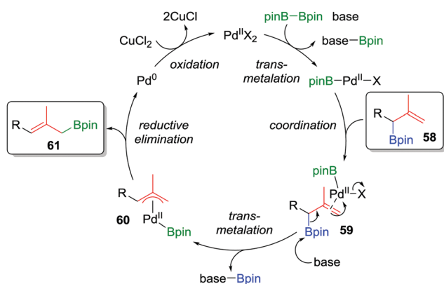
Fig. 5 Proposed mechanism of the palladium-catalyzed 1,3-rearrangement of allylic boronic esters used in a two-step three-carbon homology.
