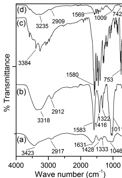
Fig. 1 FTIR spectra of (a) CMC, (b) CMC–MWCNT 3 (c) diclofenac sodium and (d) drug loaded nanocomposite.
