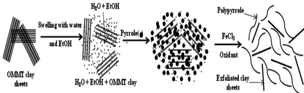
Fig. 7 The formation of exfoliated PPy-OMMTC nanocomposites. 123
