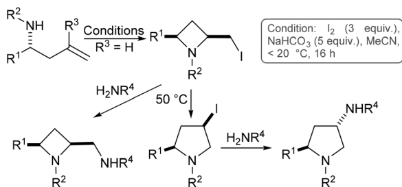
Scheme 1 Azetidines and pyrrolidines synthesis via iodine mediated cyclisation of homoallylamines (R 3 = H).
