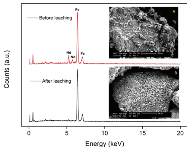
Fig. 5 SEM images (magnified 250x) and EDX spectrum of the surface of the large NdFeB particles (≈300 μm) before (A) and after (B) leaching.
