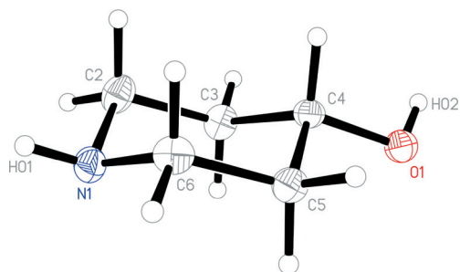
Fig. 4 The molecule of 1o in the crystal. Ellipsoids correspond to 50% probability levels.
