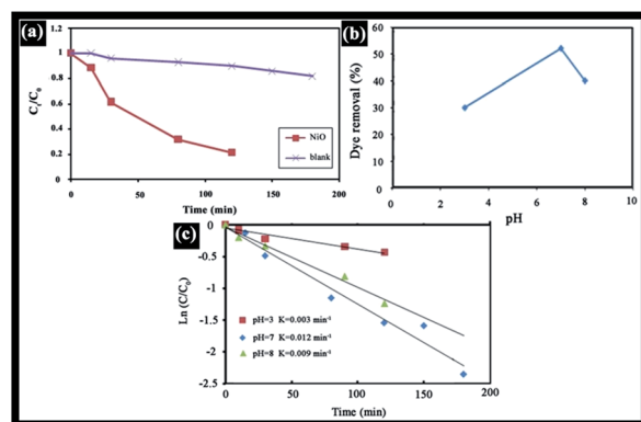
Fig. 8 (a) Variation in RB concentration with time (NiO dose ( W ) = 1 \text{ g L}^{-1} , [\text{RB}] = 10 \text{ mg L}^{-1} , pH = 7), (b) pH effect on the removal of RB dye (NiO dose ( W ) = 1 \text{ g L}^{-1} , [\text{RB}] = 10 \text{ mg L}^{-1} , T = 20^\circ \text{C} , t = 12 \text{ h} ), (c) effect of the initial pH on the photocatalytic degradation of RB dye (NiO dose ( W ) = 1 \text{ g L}^{-1} , [\text{RB}] = 10 \text{ mg L}^{-1} ).
