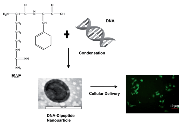
Fig. 7 Cationic dipeptide–DNA nanoparticles for cellular delivery.
