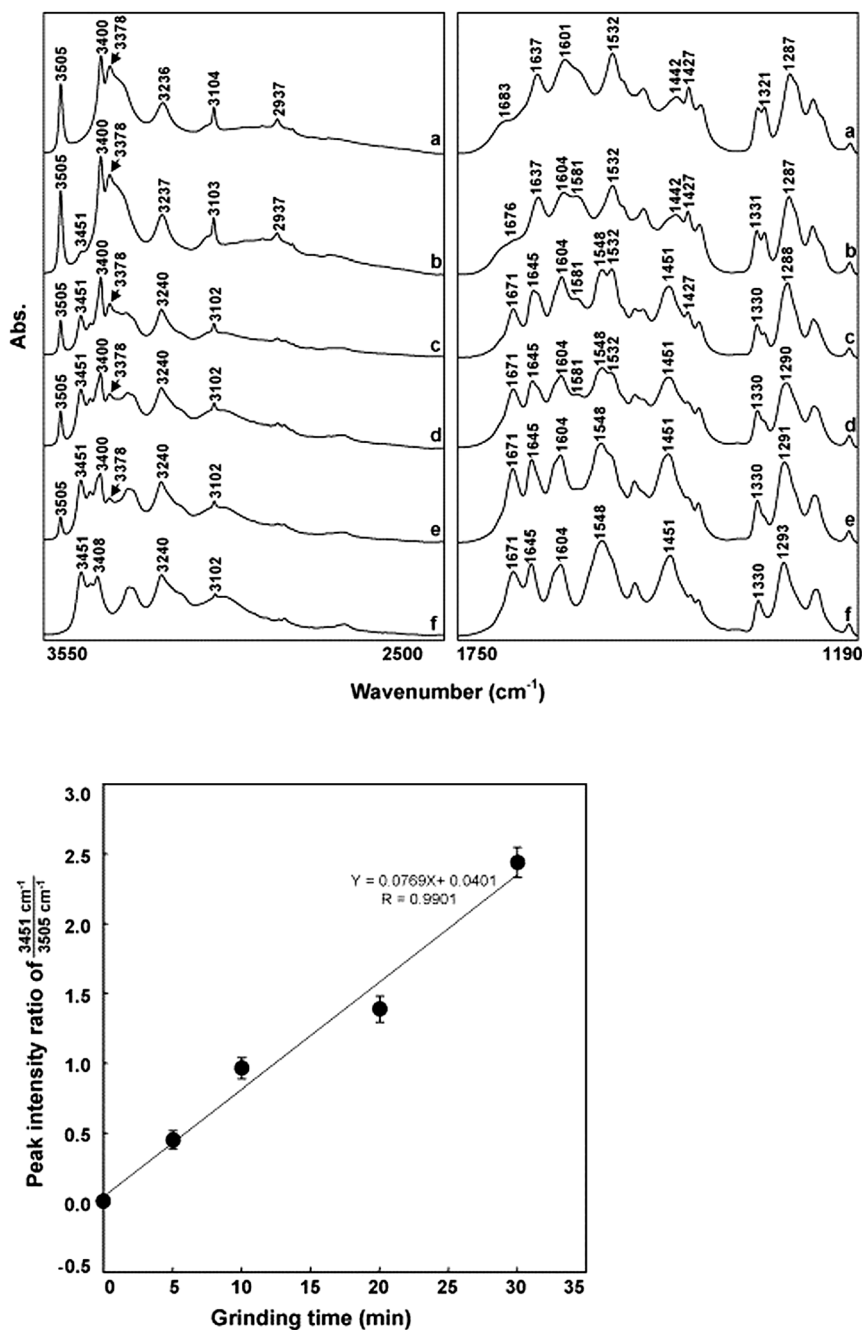
Fig. 6 (a) Grinding-time dependence of the FTIR spectra for famotidine showing from top to bottom the emergence of the absorption at 3451 cm -1 which is used to monitor the formation of Form A of the material. (b) Plot of peak intensity ratio ( I_{3451}/I_{3505} ) for the spectra above indicating a possible zero order rate law for the conversion. Reproduced from ref. 78 with permission from Elsevier.
