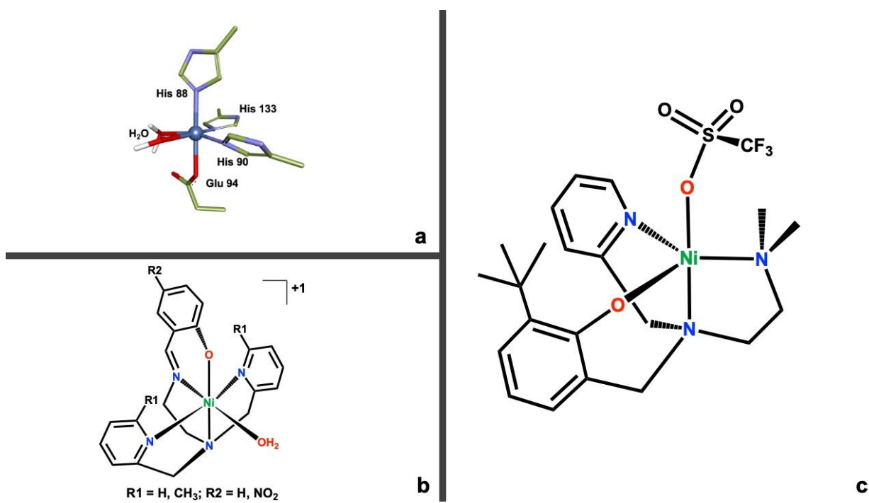
Fig. 2 a. First coordination sphere for the active site of ARD (PDB ID: 1VR3) 25 b. Structure of the first family of model complexes for ARD. 24 c. Structure of the new second generation Ni(II)N 3 O ARD model complex ( 1 ).
