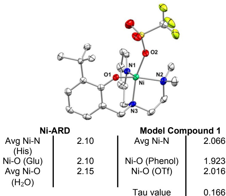
Fig. 3 Left-Crystal structure of [Ni II (N-(ethyl-N'Me 2 )(Py)(2-t-ButPhOH))(OTf)] ( 1 ) with ellipsoids drawn at the 50% probability level. H atoms omitted for clarity. Bottom- Table of selected bond lengths in Å for Ni-ARD (PDB ID: IVR3) 25 and for complex 1 .
