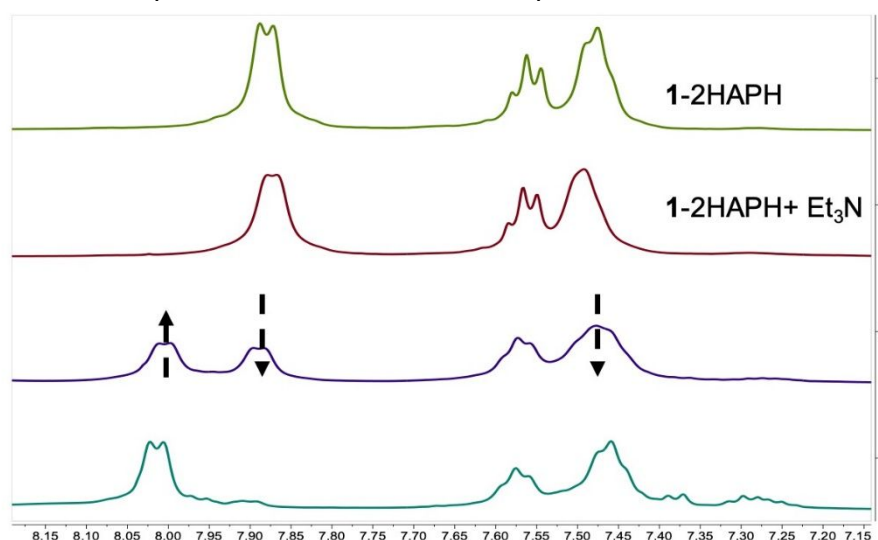
Fig. 5 1 H NMR timelapse spectra (CD 3 OD) of the aromatic region showing reactivity between complex 1 with 2HAP-H (1eq., green trace), Et 3 N (2eq., brown trace), excess O 2 (40 min. bubbling, purple trace), and final scan 180 minutes after the first addition of O 2 (teal trace) showing the complete disappearance of the starting substrate.
