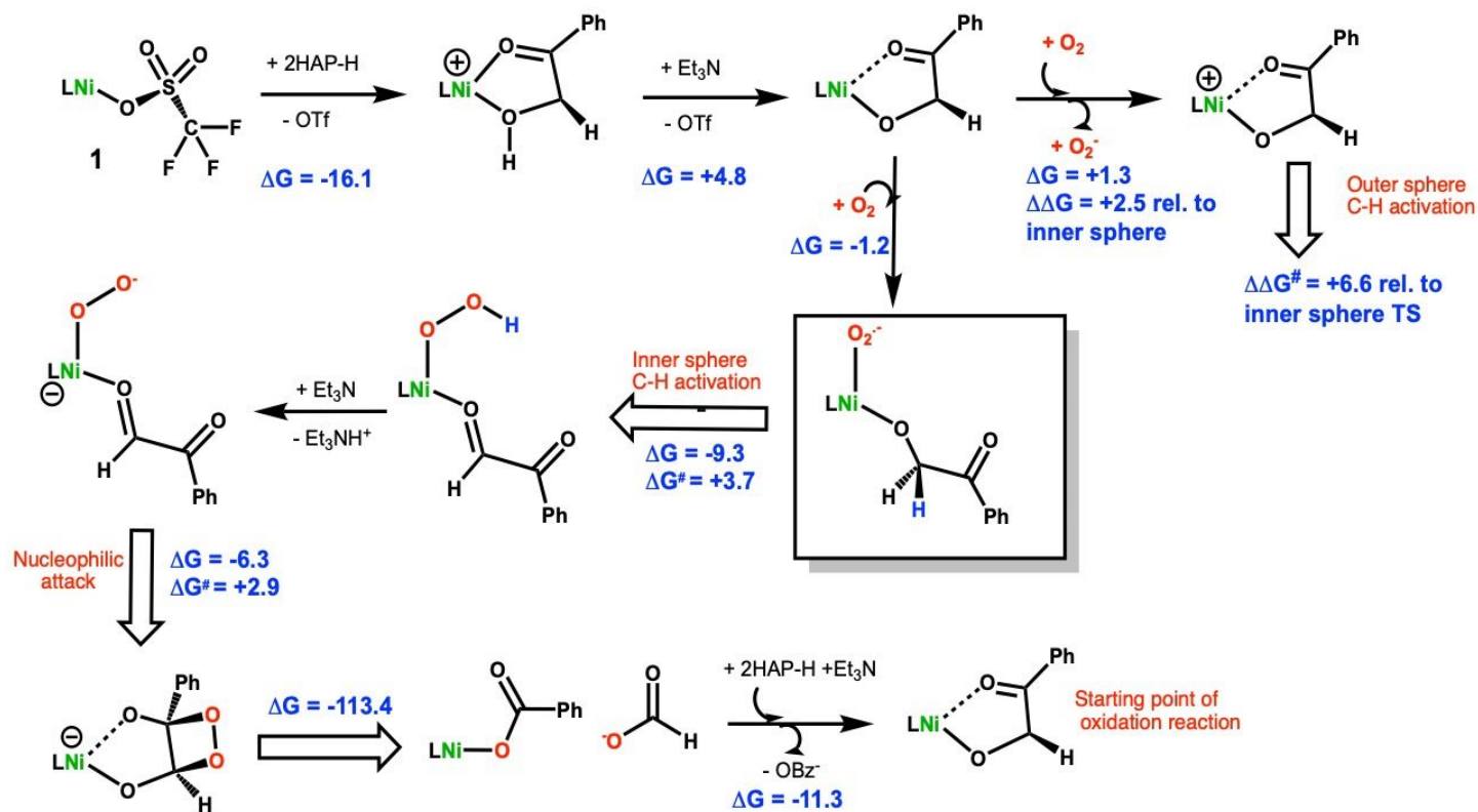
Scheme 2 Proposed reaction mechanism and relevant free energies (kcal/mol) for the O_2 mediated oxidation of 2-hydroxyacetophenone (2-HAP-H) by 1 . All nickel species are calculated to be ground state triplets with the exception of the cationic Ni(III) complexes, which are predicted to be doublets. Except for these complexes and the superoxide adduct, LNi(III)(2HAP)(O_2^-) (central box) which are best deemed as Ni(III) complexes the remaining species are best described as Ni(II). Geometries optimized at the BP86/6-31+G(d) level of theory. At those geometries, single point BP86/6-311++G(d,p) calculations are run with dispersion (GD3BJ) and solvent (SMD-methanol) corrections.
