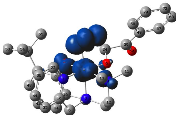
Fig. 6 Plot of spin density (IsoValue = 0.004 a.u.) of the triplet ground state of the Ni(III)-superoxide complex. Spheres: O = red, C = gray, N = blue, Ni = light blue; hydrogen atoms are omitted from the figure for clarity. Optimized bond lengths (Å): NiO 2 = 1.87, O-O = 1.30, NiO alkoxide = 1.88, NiN amine (trans to phenolate) = 2.50, NiN py = 1.97, NiO phenolate = 2.05, NiN amine (trans to O 2 ) = 2.05. Ligand-metal-ligand angles = 90 ± 10°.
