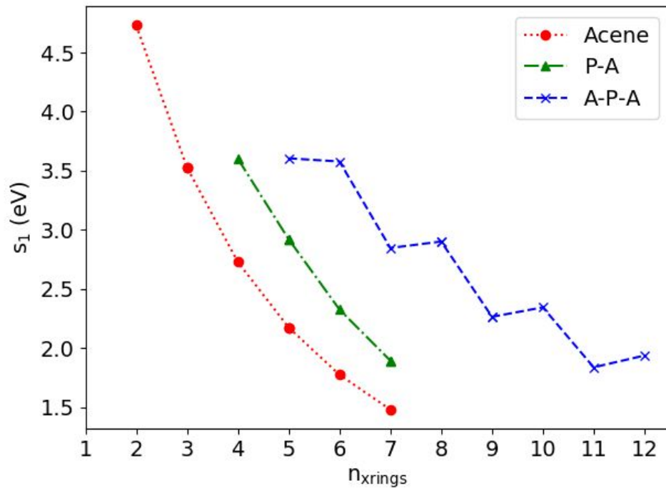
Figure 4. \epsilon^{S_1} as a function of n_{\text{xrings}} for acenes, P-A and A-P-A as determined via TDDFT at the (OT)-LC- \omega HPBE/Def2TZVP level of theory.
