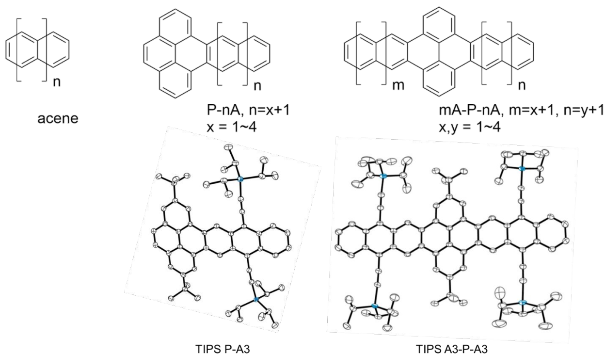
Figure 1. Molecular structures and their abbreviations used throughout this study. (top) Molecules used in theoretical calculations (bottom) Thermal ellipsoids of pyrenoanthracene (TIPS P-A3) and pyrenodianthracene (TIPS A3-P-A3).
