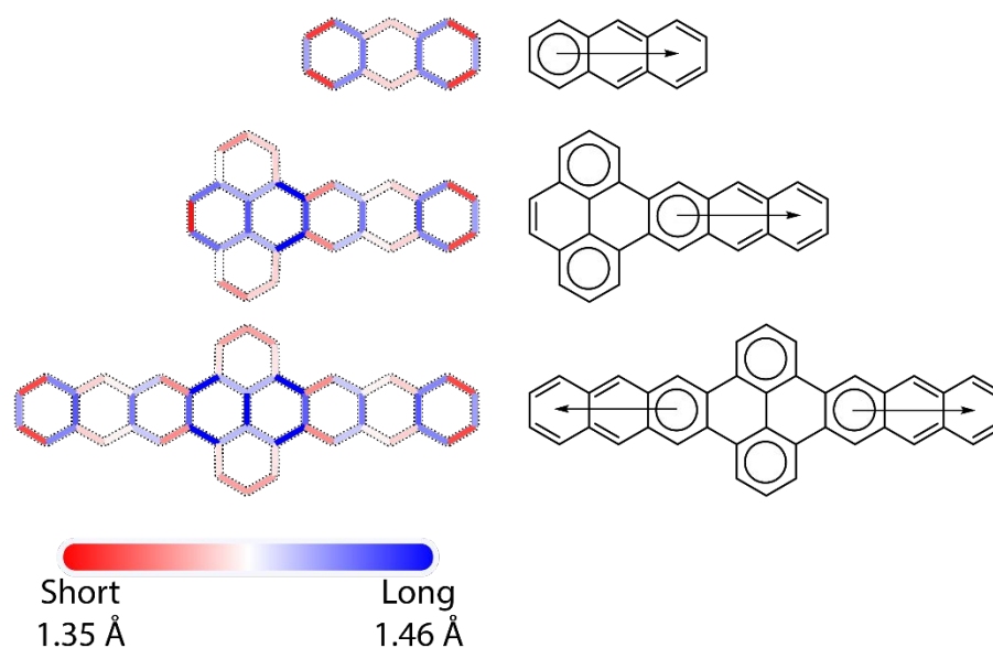
Figure 2. (Left) Bond length alternation (BLA) patterns of, from top to bottom, anthracene, P-A3, A3-P-A3 as determined at the LC- \omega HPBE/Def2TZVP level of theory. Only the C-C bonds in the molecular backbones are shown. (Right) Corresponding Clar formulae of these molecules.
