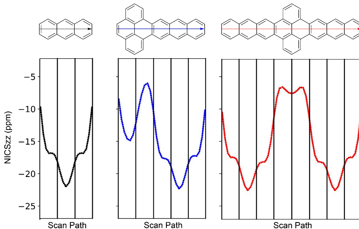
Figure 3. NICS-xy scan of anthracene, P-A3, and A3-P-A3 as determined at the LC- \omega HPBE/Def2TZVP level of theory. For each molecule, the scan path consists of points on a straight line running from the left end to the right end.
