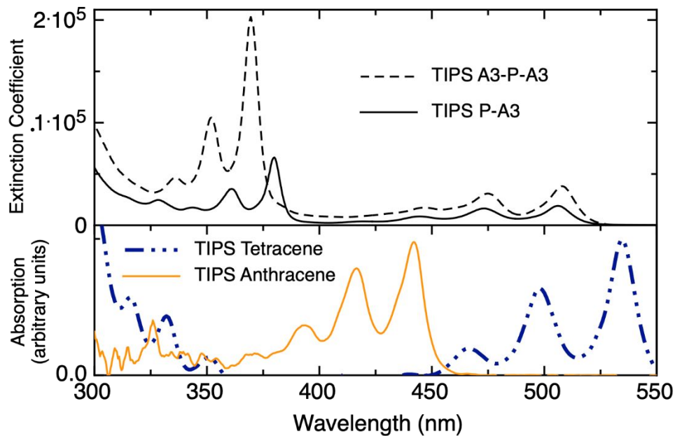
Figure 5. UV-vis Absorption spectra of TIPS anthracene, TIPS tetracene, TIPS P-A3, and TIPS A3-P-A3. The absorption for TIPS P-A3 is red-shifted compared to TIPS anthracene, but blue-shifted to TIPS tetracene.
