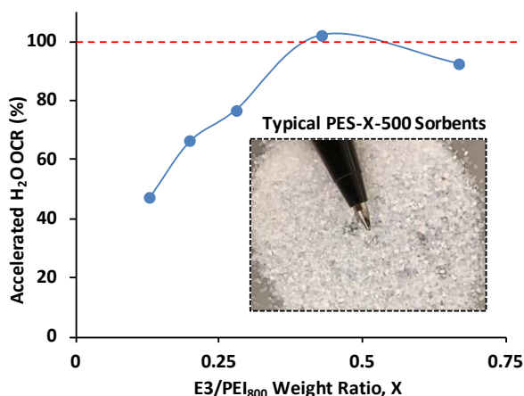
Fig. 2. OCR values for 500 \mu\text{m} , PES-X-500 sorbents. The inset picture shows the external morphology of the irregularly shaped particles.
