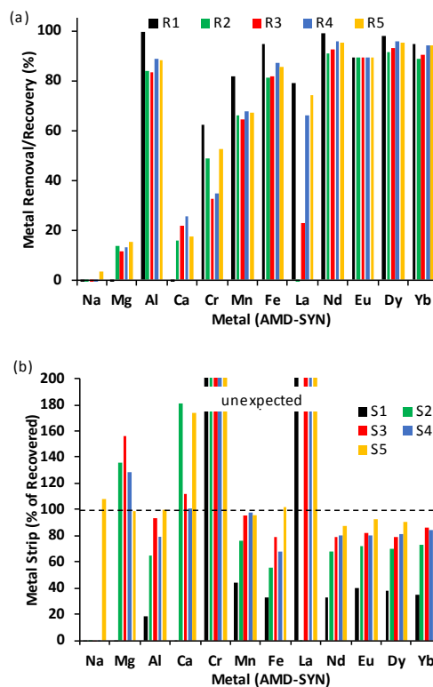
Fig. 8: Cyclic metal recover-strip (a)-(b) testing with synthetic acid mine drainage, AMD-SYN – 354 ppm alkali plus alkaline metals, 341 ppm heavy metals, 53.9 ppb REEs, pH 2.6, fouling (alkali+alkaline+heavy)/REE ratio of 12,892/1.
