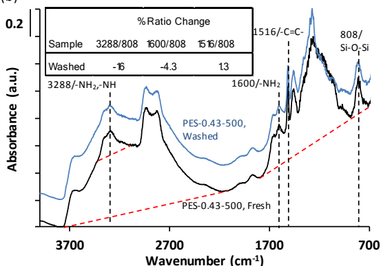
Fig. 3: (a) PEI 800 concentration profile during PES-0.43-500 washing, determined by a UV-Vis/Cu 2+ technique. (b) DRIFTS absorbance spectra of fresh and washed sorbent, taken at 50 °C. Absorbance=log(1/I), where I is the single beam spectrum of each sample pretreated at 120 °C in N 2 for 30 min then cooled down.
