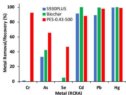
Fig. 5: Removal of toxic, aqueous cationic and oxyanionic RCRA heavy metals from a 160 ppm-concentrated solution at pH 6.24 by different sorbent types.
