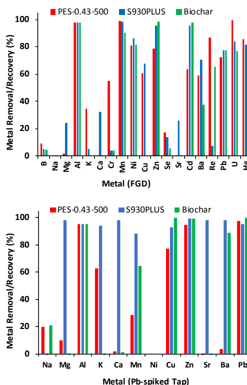
Fig. 6: Removal of RCRA and other heavy metals from (a) flue gas desulfurization water – 2,606 ppm alkali plus alkaline metals, 121.3 ppm heavy metals, 1.6 ppb REEs, pH 6.7;
