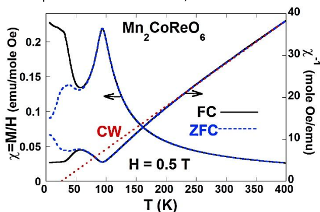
Figure 2. The H=0.5 T, temperature dependent magnetic susceptibility, \chi , and the inverse susceptibilities, \chi^{-1} , for Mn_2CoReO_6 collected under field cooled (FC) and zero field cooled (ZFC) conditions. The Curie Weiss (CW) fit to the high temperature \chi^{-1} data is indicated by a dotted line.
