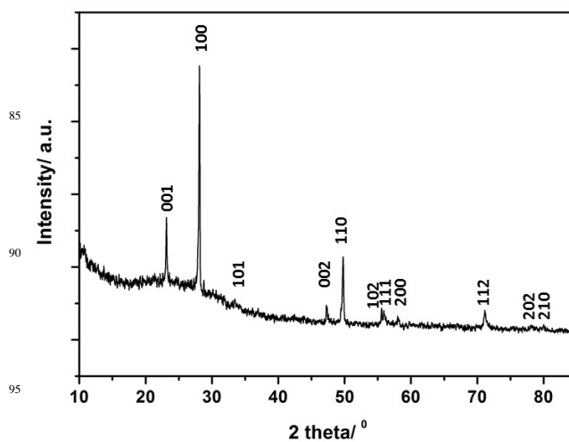
Fig. 2 Typical XRD pattern of a Li 3-x-y M x N sample (M= Co-Cu) synthesised by MW methods (sample 2 is shown). Indices for the expected reflections are indicated.
