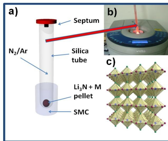
Fig. 1 (a) Schematic experimental configuration for the SMC MW synthesis of lithium nitridometallates; (b) Image of reaction in progress; and (c) Polyhedral representation of \text{Li}_{3-x-y}\text{M}_x\text{N} , where M = \text{Co-Cu} . N (blue spheres); Li(2) (pink spheres); and Li(1) (green spheres).
