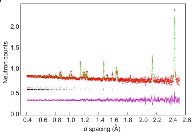
Fig. 3 Rietveld fit against PND data collected at room temperature from sample 4 in the 2\theta = 145^\circ (backscattering) detector bank. Observed data points are shown in red, calculated profile in green and the difference (obs-calc) profile in pink. Black and red vertical tick marks indicate reflections from the \text{Li}_{3-x-y}\text{Co}_x\text{N} phase and the vanadium sample can respectively.
