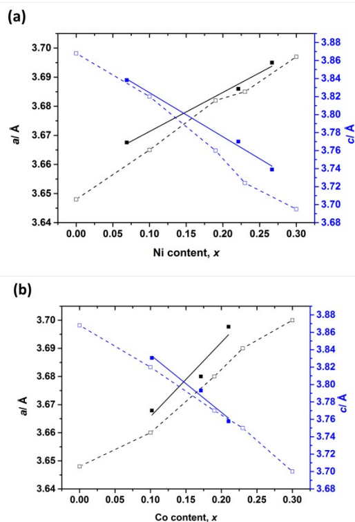
Fig. 4 Variations of unit cell parameters with varying (a) Ni (1-3) and (b) Co (4-6) substitution levels ( x ). Filled squares show refined values from our PND data. Empty squares show data from reference 11. Trend lines serve as a guide to the eye.
