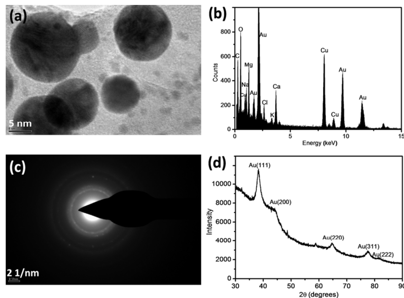
Fig. 7. TEM image (a) of the Au nanoparticles produced in the Chaobai river water under sunlight irradiation with the corresponding EDS (b) and SAED pattern (c) of the Au nanoparticles. The result of XRD of the as-prepared Au nanoparticles in the Chaobai river water 1 under sunlight irradiation is also shown (d). The concentration of spiked \text{AuCl}_4^- is 200 \mu\text{mol L}^{-1} and cumulative parabolic aluminized reflector is 7.06 \times \text{m}^{-2} (corresponding to 3 h sunlight irradiation). (EDS - Energy-dispersive X-ray spectroscopy; SAED Selected-area electron diffraction – XRD – X-ray diffraction) (Adapted with permission from Ref 30 copyright American Chemical Society).
