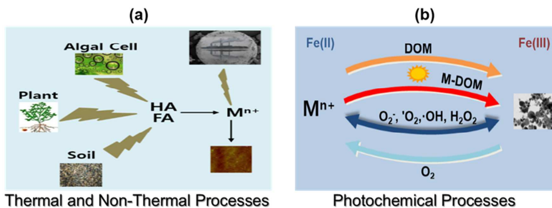
Fig. 2. (a) Thermal and non-thermal processes and (b) photochemical processes that generate natural nanoparticles in the environment (for details see section 2). (HA-humic acid; FA-fulvic acid; DOM-dissolved organic matter; M^{n+} - Metal ions (e.g. Ag(I) and Au(III)); M-DOM – Metal ions complexation with dissolved organic matter).
