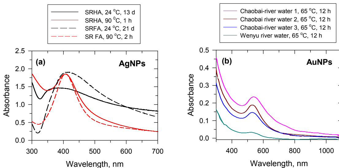
Fig. 5. (a) UV-vis absorption spectra of Ag nanoparticles (AgNPs) in Suwannee river humic acid (SRHA) and Suwannee river fulvic acid (SRFA) at 24 °C and 90 °C at pH 8.0 ( [Ag^+] = 1 \times 10^{-4} \text{ mol L}^{-1} , [SRFA] = [SRHA] = 100 \text{ mg L}^{-1} ). (Adapted with permission from Ref 12 copyright American Chemical Society). (b) UV-Vis absorption spectra of Au nanoparticles (AuNPs) in river water at 65 °C at pH 8.0 ( [Au^+] = (62.5-1000) \times 10^{-6} \text{ mol L}^{-1} , [HA] = 5-100 \text{ mg DOC L}^{-1} , where DOC – Dissolved organic carbon). (c) (Adapted with permission from Ref 30 copyright American Chemical Society).
