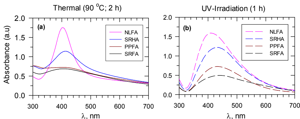
Fig. 9. UV-Vis absorption spectra of Ag nanoparticles for different fulvic acids and Suwannee river humic acid at pH 8.0. Adapted with permission from Ref 12, 13 , copyright American Chemical Society). (a) Heating at 90 °C for 2 h and (b) UV irradiation for 1 h for in moderately hard reconstituted water (MRHW) synthetic freshwater. (SRFA – Suwannee river fulvic acid I, SRPP – Suwannee river Pahokee Peat II, SRNL – Suwannee river Nordic Lake; SRHA – Suwannee river II humic acid) ( [\text{Ag}^+] = 1 \times 10^{-3} \text{ mol L}^{-1} , 45 mg L -1 fulvic and humic acids).
