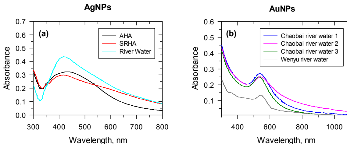
Fig. 6. UV-vis spectra of nanoparticles formed in river water conditions. (a) Ag nanoparticles, 4 mg L -1 Suwannee river humic acid (SRHA) (red lines), or 4 mg L -1 C/L Aldrich humic acid (AHA) (black lines) upon exposure to stimulated sunlight in the CPS+ reactor for 20 min. ([Ag + ] = 1 × 10 -4 M; pH 8.0). (Adapted with permission from Ref 28 , copyright American Chemical Society). (b) Au nanoparticles under natural sunlight. (Cumulative parabolic aluminized reflector (PAR) light = 12.48 E m -2 ). (Adapted with permission from Ref 30 , copyright American Chemical Society).
