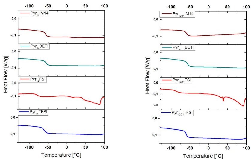
Figure 4: DSC of polymer electrolytes, 5 \text{ K min}^{-1} , 1 st heating scan, exothermic heat up.
