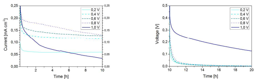
Figure 8: Chronoamperometry curves at various voltages (left panel) as detected upon 10 h polarization steps applied to the Pyr 14 TFSi-containing polymer electrolyte in symmetric lithium cells (T= 40°C). The cell voltage relaxation recorded during the intermixed rest steps are also reported (right).
