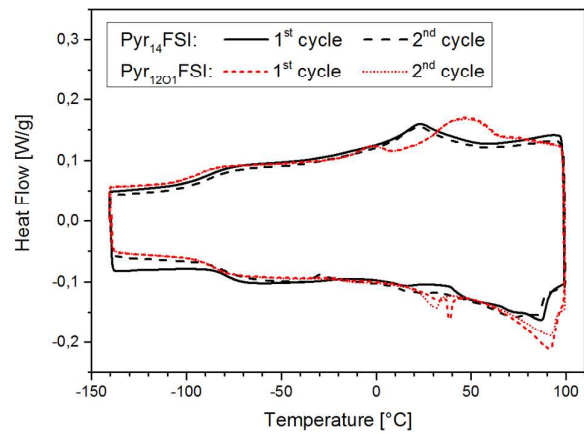
Figure 6: DSC curves of Pyr 14 FSI- and Pyr 1201 FSI-containing electrolytes, 1 st and 2 nd heating/cooling cycle, exothermic heat up.
