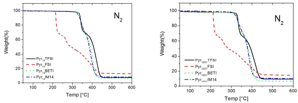
Figure 2: TGA of polymer electrolytes in inert atmosphere. Scan rate 5°C min -1 .
