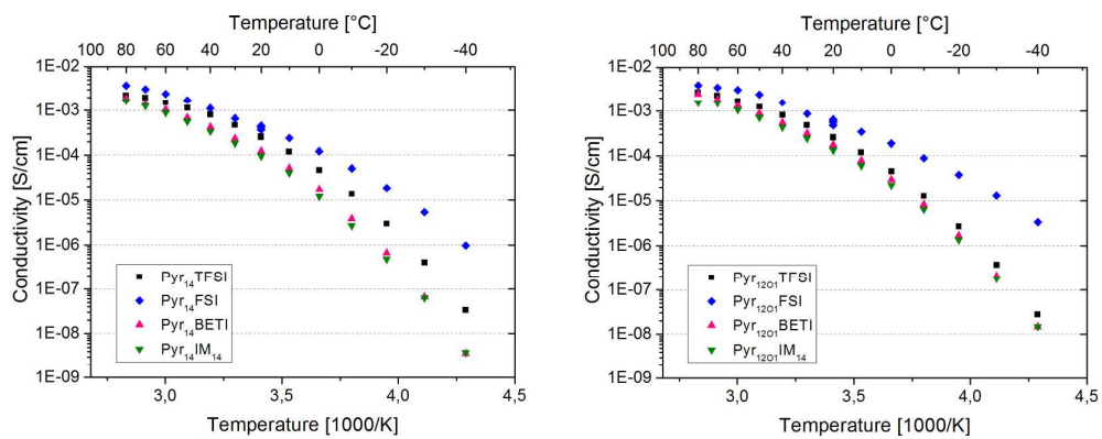
Figure 5: Arrhenius plot for Pyr 14 - (left side) and Pyr 1201 - (right side) containing electrolytes.
