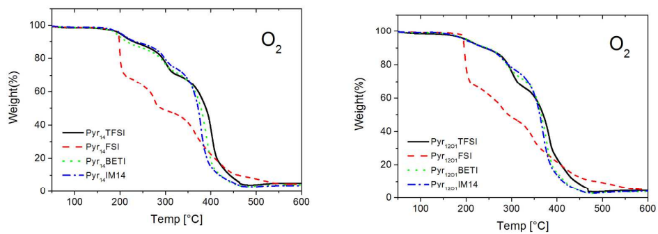
Figure 3: TGA of the polymer electrolytes in oxygen atmosphere. Scan rate 5^{\circ}\text{C min}^{-1} .
