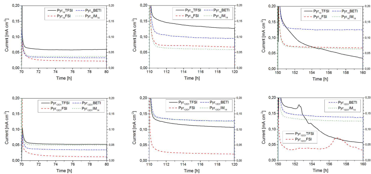
Figure 7: Chronoamperometry curves upon 10 h polarization steps (intermixed with 10 h relaxation steps) at 0.2 V (left), 0.6 V (center) and 1.0 V (right); Pyr 14 - containing electrolytes (top) and Pyr 1201 - containing electrolytes (bottom). All measurements were performed at 40 °C.
