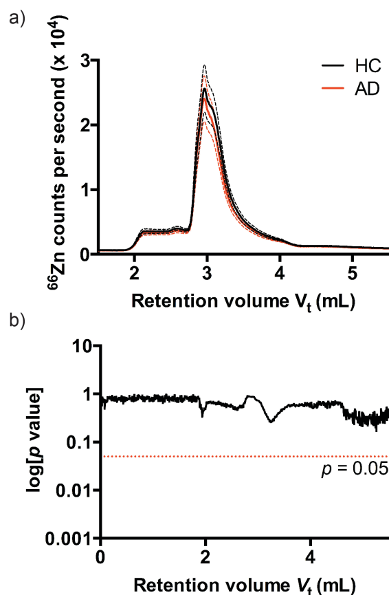
Fig. 2 (a) SEC-ICP-MS chromatograms of mean ^{66}\text{Zn} signal (solid line, \pm 1 SD dashed lines) in 38 AD and 38 HC subjects. (b) A two-tailed t -test on each point revealed no significant difference between groups.
