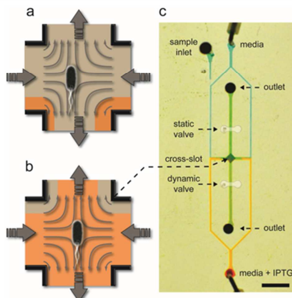
Fig. 2 Microfluidic device and schematic of trapping mechanism in the SCM. (a,b) Schematics of cell confinement in cross-slot region (not to scale), and the transitioning of growth environments from Medium A to Medium B. (a) A single cell is initially grown in Medium A (tan color), followed by (b) rapid switching of the cell environment to Medium B (orange color) while confining the cell in free solution (see Movie S1). (c) Optical micrograph of the SCM. Scale bar: 3 mm.
