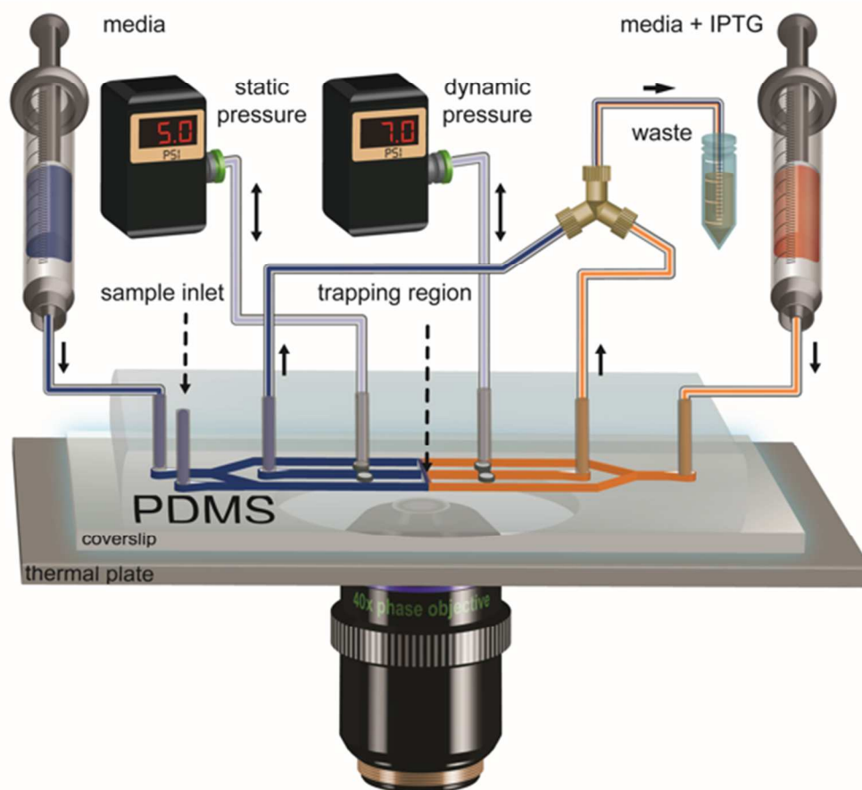
Fig. 1 Schematic of single cell microbioreactor (SCM). The integrated device consists of several key components including: computer-controlled pressure regulators for controlling valve pressure, computer-controlled syringe pumps for delivering media into the device, and a thin-film thermal plate heater positioned underneath the device with thermocouple for controlling the temperature. The microfluidic platform is mounted on an inverted microscope equipped for phase-contrast and fluorescence imaging. The device allows for two distinct inlet media streams with a separate inlet for delivery of sample. Device components are integrated and controlled using a custom LabVIEW program.
