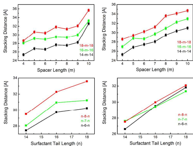
Figure 4: Graphical presentation of the d -values corresponding to the first observable stacking reflection in the PXRD measurements of all synthesized MIF materials as a function of spacer length (top) and tail length (bottom). Left: IM bridged MIFs, right: MeIM bridged MIFs.
