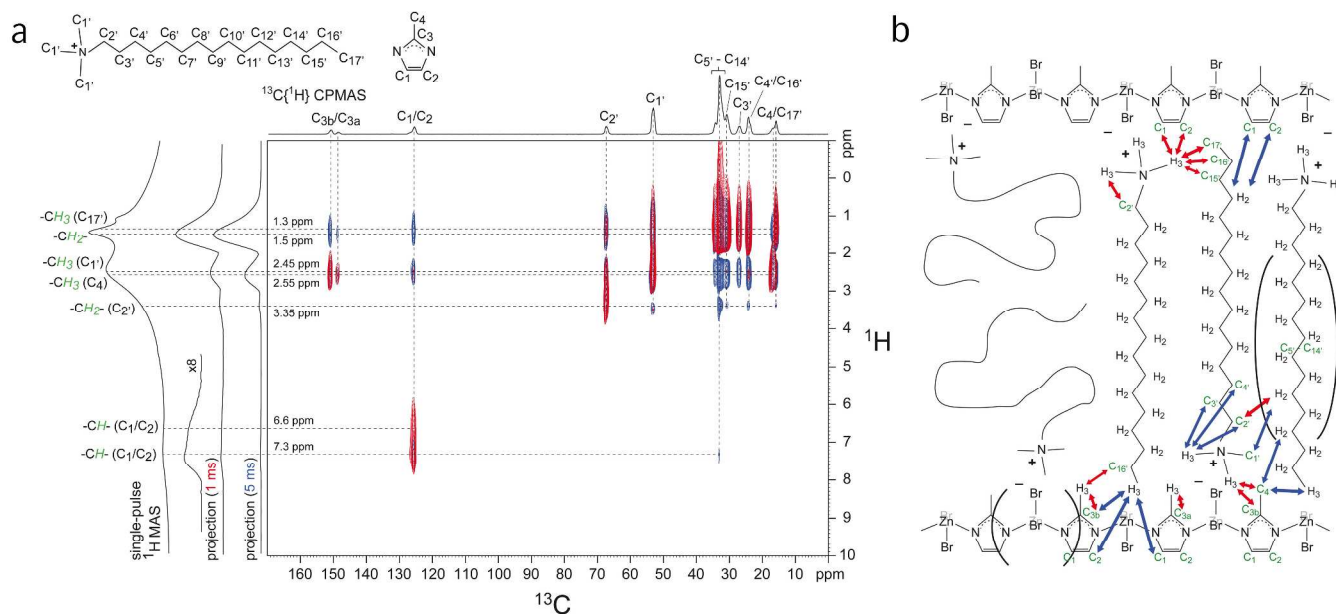
Figure 5: (a) Solid-state 2D ^{13}\text{C}\{^1\text{H}\} HETCOR NMR spectra acquired at room temperature for as-synthesized MIF-1 under MAS conditions of 12.5 kHz with 1 ms (red) or 5 ms (blue) cross-polarization (CP) contact times. For comparison, 1D single-pulse ^1\text{H} MAS and 1D ^{13}\text{C}\{^1\text{H}\} CPMAS spectra are shown along the vertical and horizontal axes, respectively, of the 2D spectra. Schematic diagrams of the \text{CTA}^+ surfactant and methylimidazole molecules are shown and their corresponding ^{13}\text{C} and ^1\text{H} signal assignments are indicated in the 1D spectra. (b) Schematic diagram of MIF-1 (Zn/MeIM/CTAB) showing interactions between the zinc imidazolate chains and the \text{CTA}^+ molecules that are consistent with the 2D ^{13}\text{C}\{^1\text{H}\} HETCOR NMR analyses. Carbon and hydrogen atoms are labeled according to the assignments in Figure 1. Red and blue arrows indicate ^{13}\text{C} - ^1\text{H} dipolar interactions at short (1 ms) and long (5 ms) contact times, respectively. Note that Zn and Br atoms oriented into the page are colored gray. A fraction of the \text{CTA}^+ molecules are thought to be interdigitated with an antiparallel stacking arrangement.
