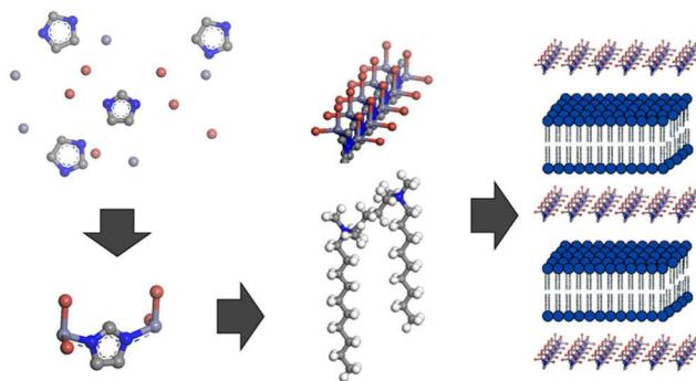
Figure 6: Proposed formation of MIF materials by electrostatically-driven cooperative self-assembly. Upon addition of bromide to the solution containing imidazole, zinc and the surfactant, one-dimensional chains form and arrange into quasi two-dimensional layers, intercalated by surfactant ions for charge compensation. Note that the surfactants are omitted on the left-hand side for clarity.
