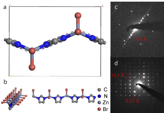
Figure 2: (a) Structure model of the zinc imidazolate bromide chain viewed along the b -axis and (b) along / onto the chains. (c,d) TEM SAED images of 16-6-16 IM MIF (c) perpendicular to the [010] direction and (d) of the (101) plane.
