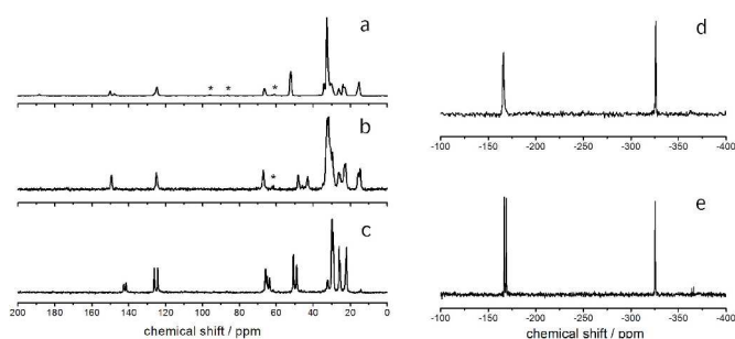
Figure 3: Solid-state ^{13}\text{C} MAS NMR spectra of (a) MIF-1, [20] (b) 16-10-16 MeIM MIF and (c) 14-6-14 IM MIF and solid-state ^{15}\text{N} MAS NMR spectra of (d) 16-10-16 MeIM MIF and (e) 14-6-14 IM MIF. Asterisks indicate spinning side bands.
