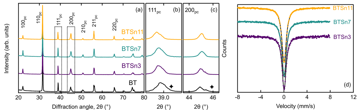
Fig. 1 Room temperature X-ray diffraction measurement of sintered BTSn100x with (a) the full measurement range and the enlarged reflections (b) 111_{pc} , and (c) 200_{pc} (pc:pseudo-cubic). The K\alpha_2 contribution is marked with a star. ^{119}\text{Sn} Mössbauer spectroscopy (d) with Lorentzian fit (black) of sintered and crushed sample, revealing a \text{Sn}^{4+} oxidation state.
