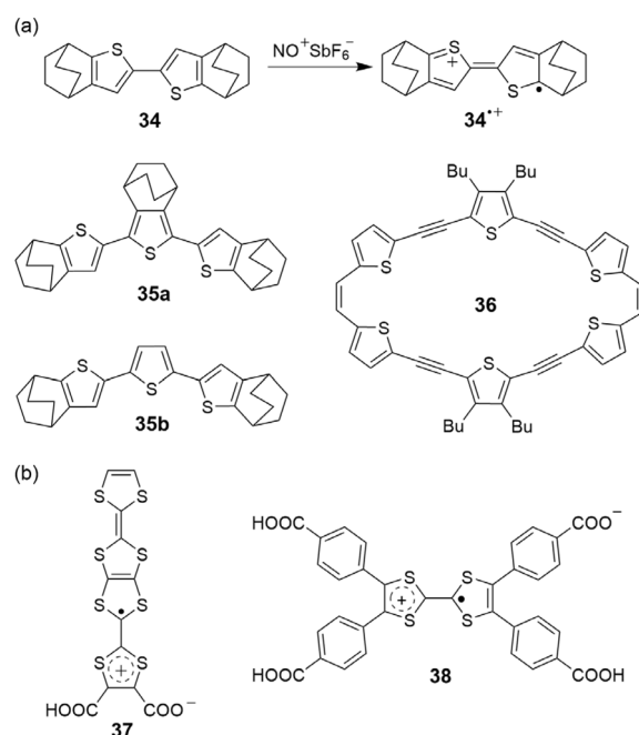
Fig. 12 (a) Thiophene-containing molecules; (b) TTF-containing zwitterions.
