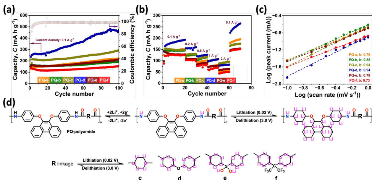
Fig. 3 (a) Cycling performance measured at a current density of 0.1 \text{ A g}^{-1} ; (b) rate capability evaluated at different current densities ranging from 0.1 to 2.0 \text{ A g}^{-1} ; (c) b -value determination based on the relationship between peak current and scan rate; and (d) schematic illustration of the lithium-ion storage mechanism in PQ-polyamides, highlighting \text{Li}^+ coordination with heteroatoms and \text{Li}^+\text{--}\pi interactions within the conjugated backbone and substituent-derived aromatic systems.
