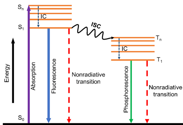
Fig. 2 Schematic diagram of the fluorescence and phosphorescence emission mechanism. Abbreviations: IC, internal conversion; ISC, intersystem conversion.
