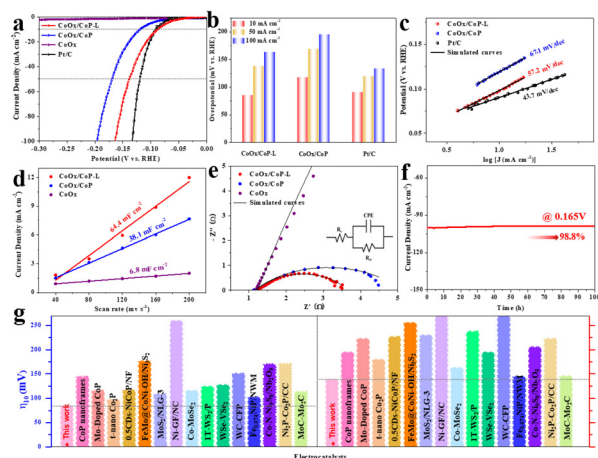
Fig. 5 HER electrocatalytic properties of CoOx/CoP, CoOx/CoP-L, CoOx precursor and Pt/C in 0.5 M H 2 SO 4 : (a) LSV curves, (b) comparison diagram of voltage at current densities of 10, 50, and 100 mA cm -2 , (c) Tafel slopes, (d) C dl curves, (e) Nyquist plots at a specific voltage of -0.15 V, (f) chronoamperometry test of CoOx/CoP-L and (g) comparison diagram of recently reported non-noble-metal-based electrocatalysts.
