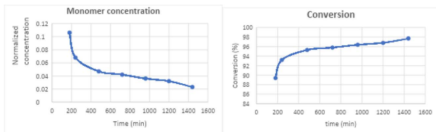
Fig. 4 Homopolymerization of P2VVPS in a continuous flow reactor set-up: flow 0.2 \text{ ml min}^{-1} up to 1 \text{ ml min}^{-1} using a step of 0.1 \text{ ml min}^{-1} showed the correlation of monomer concentration and the conversion percentage in a quiescent experiment under ambient time and pressures.
