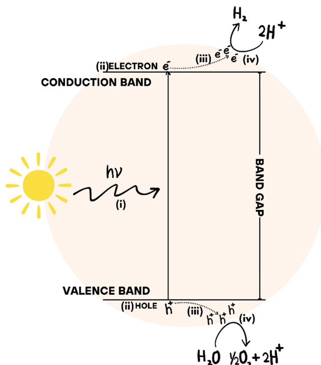
Fig. 3 Key steps involved in the photocatalytic water-splitting process: (i) photon absorption; (ii) electron-hole generation; (iii) carrier separation and migration; and (iv) redox reactions at the surface.
