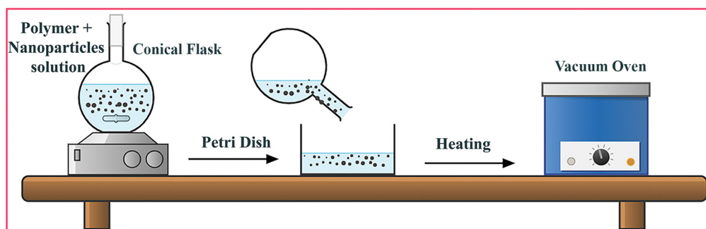
Fig. 7 Schematic illustration of the preparation procedure of an inorganic particle-filled composite membrane.
