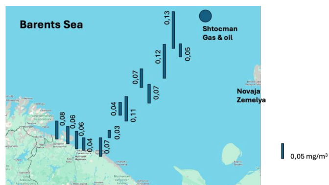
Figure 18: Distribution of petroleum hydrocarbons in the surface waters [ \text{mg/m}^3 ] along the projected Stockman pipeline. Report IMR/PINRO; Joint report Barents Sea 2007
